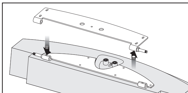
Figure 11. Reinstall the two set screws to hold hinge pins in place.
