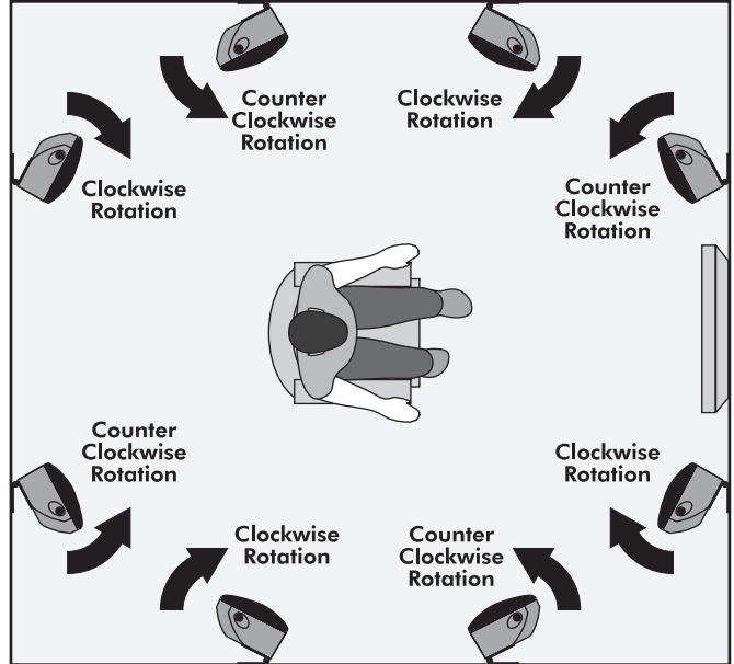
Figure 3. Vertical Installation. Rotation direction for various installation
