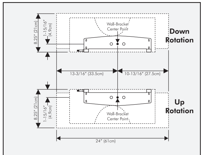
Figure 17. Determining the wall brackets center point in a horizontal
