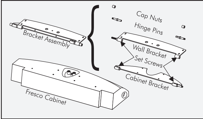
Figure 2. The parts of the Fresco i bracket assembly.
