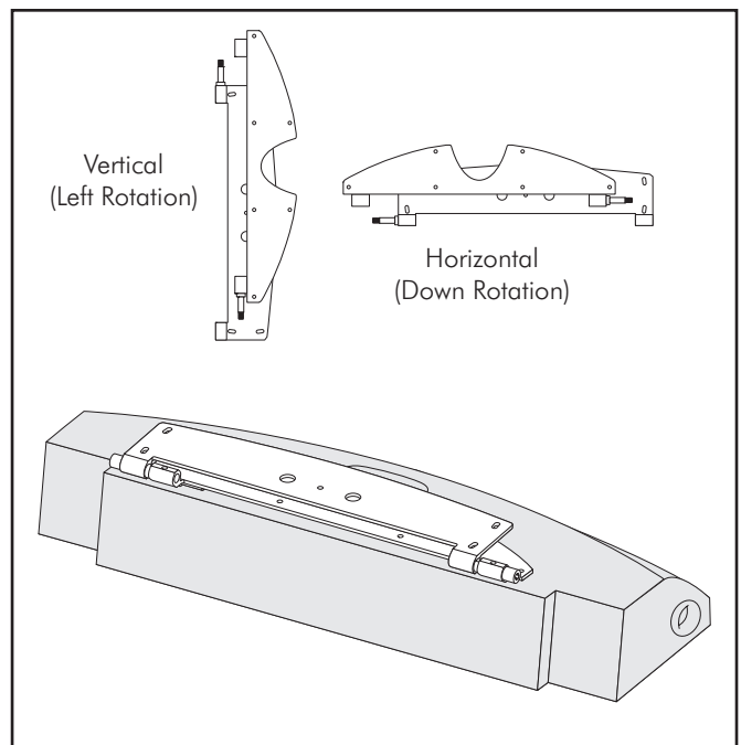
Figure 6. Fresco i's bracket assembly configured for left/down rotation
