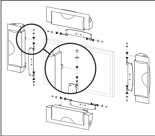
Figure 23. Install the Fresco i and the washers and cap nuts.
