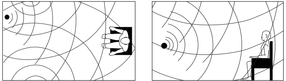
Figure 11–12. As can be seen here, point source concepts invite a great deal of room interaction. While delivering good frequency response to a large listening audience, imaging is consequently confused and blurred.
