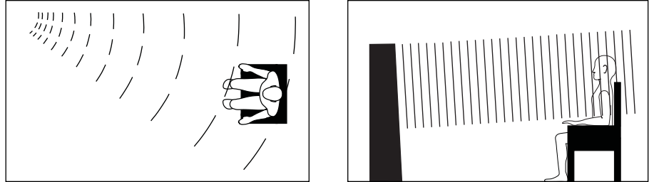
Figure 13–14. Even though they suffer from “venetian blind” effect, angled multiple panel speakers can deliver good imaging, but only to specific spots in the listening area.
