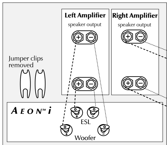
Figure 5. Vertical passive bi-amplification. One channel shown.
