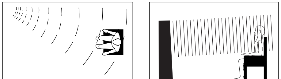
Figure 11–12. Even though they suffer from “venetian blind” effect, angled multiple panel speakers can deliver good imaging, but only to specific spots in the listening area.
