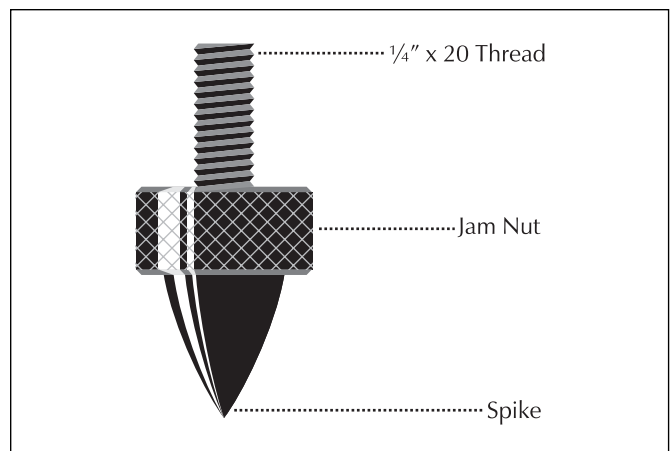
Figure 4. The ETC Spike.
