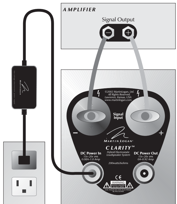
Figure 1. Single-wire and power connection. One channel shown.
