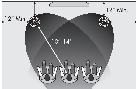
Figure 2. 2-channel installation.
