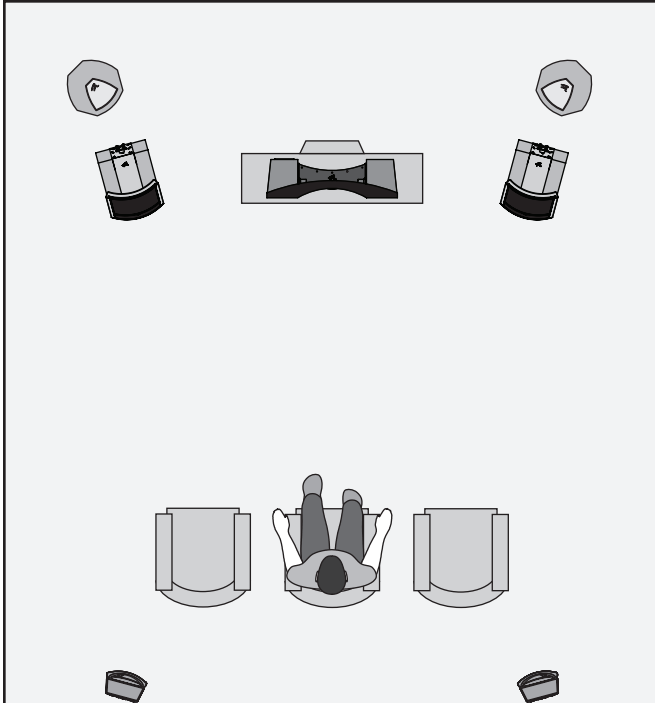
Figure 11. Montis speakers as front channels, MartinLogan electrostatic speakers as center and surround (effects) channels, and MartinLogan subwoofers as LFE (effects) channel.
