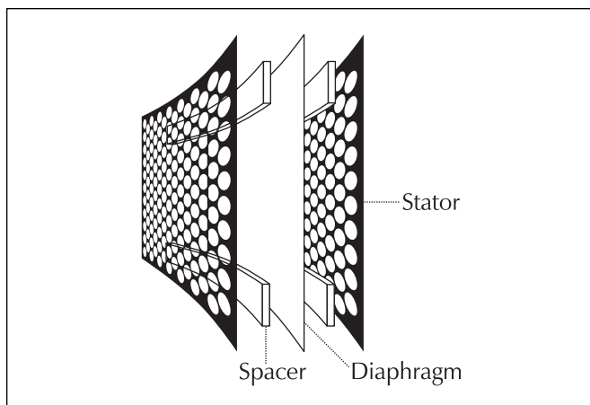
Figure 25. Cut away view of an electrostatic transducer. Notice the simplicity due to minimal parts usage.
