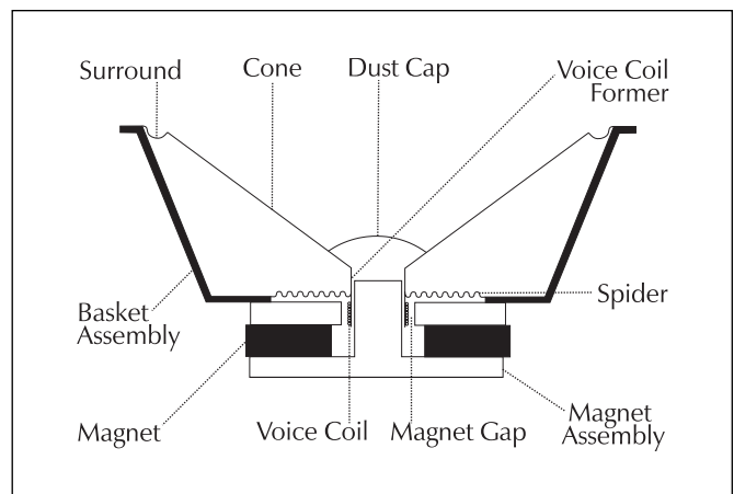
Figure 26. Cut away view of a typical moving coil driver. Notice the complexity due to the high number of parts.
